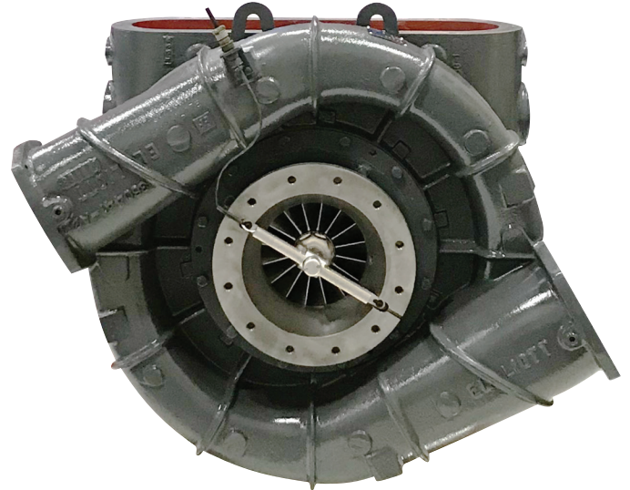
Upgraded Elliott BC370H Turbocharger
