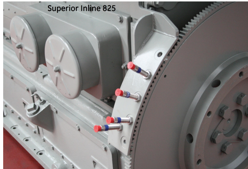
Magnetic pick-up mounting bracket on Superior 825 Inline engine
