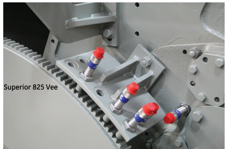
Right bank magnetic pick-up mounting bracket on Superior 825 Vee engine
